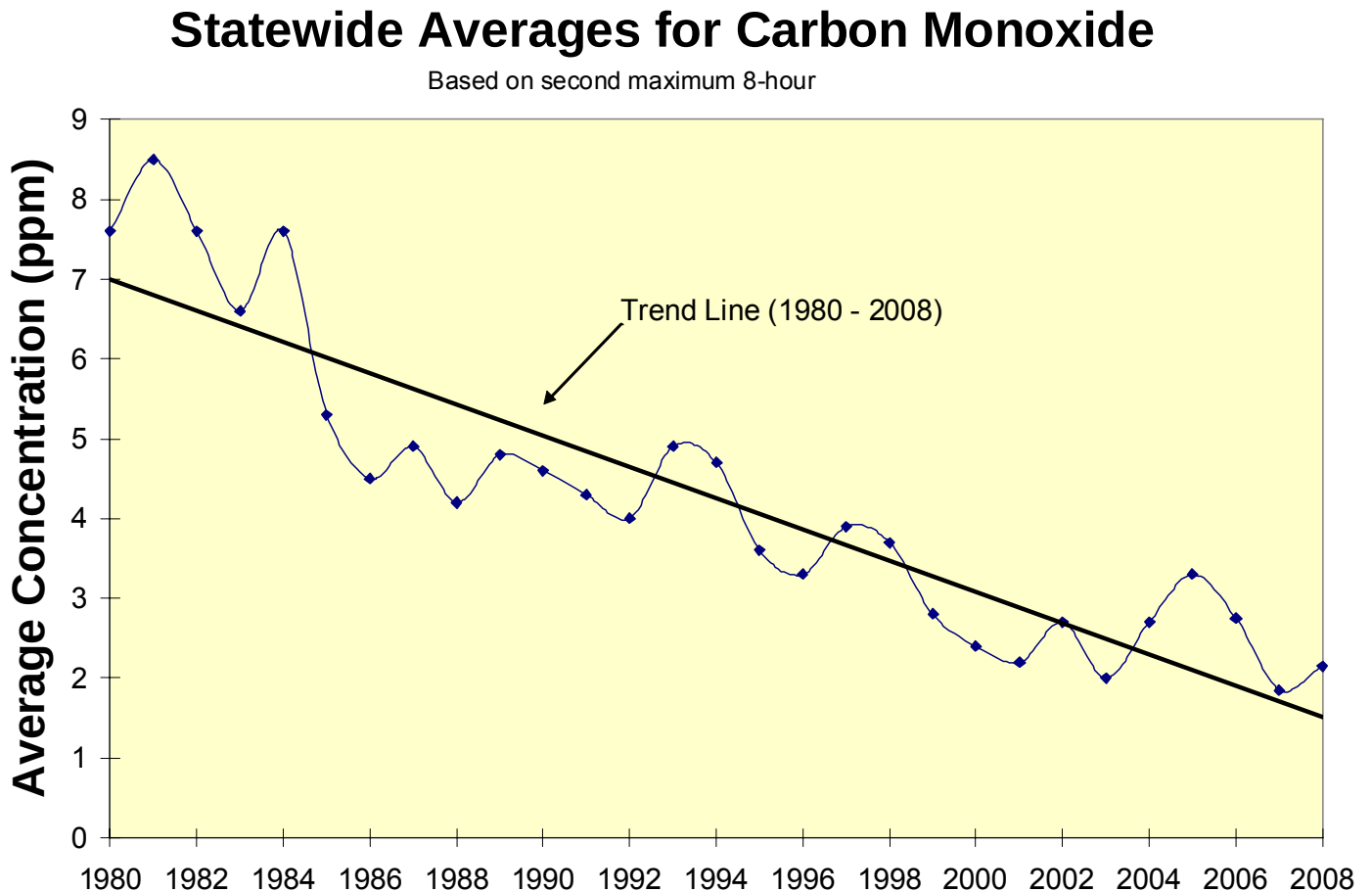
Figure 30: Statewide averages for CO monitoring indicate pollution reductions.
