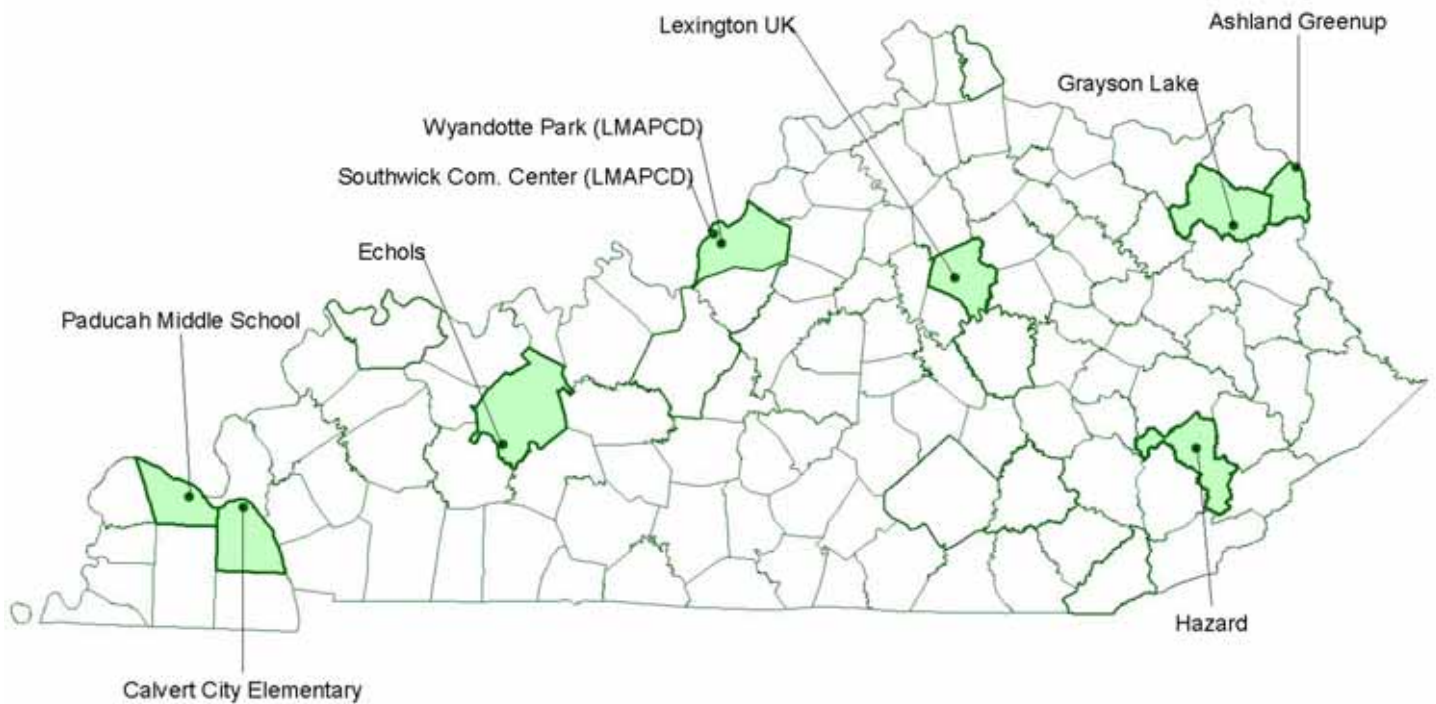
Figure 39: PM 10 monitoring locations in Kentucky.
