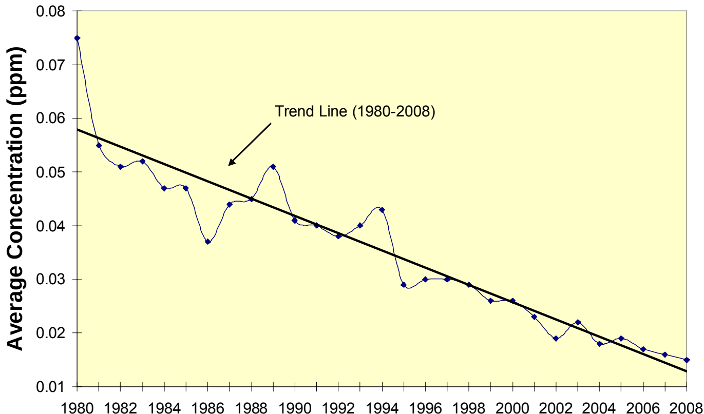
Figure 42: Statewide averages for SO 2 monitoring indicate pollution reductions.
