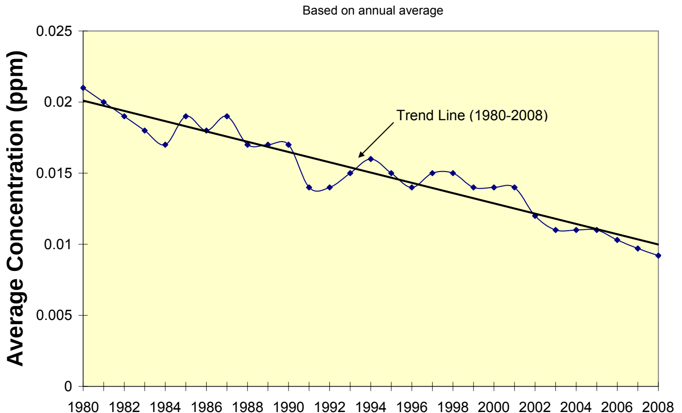
Figure 33: Statewide averages for nitrogen dioxide monitoring indicate pollution reductions.
