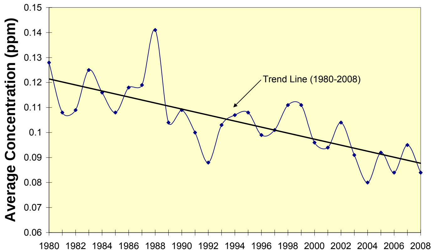
Figure 35: Statewide averages for ozone monitoring indicate pollution reductions.
