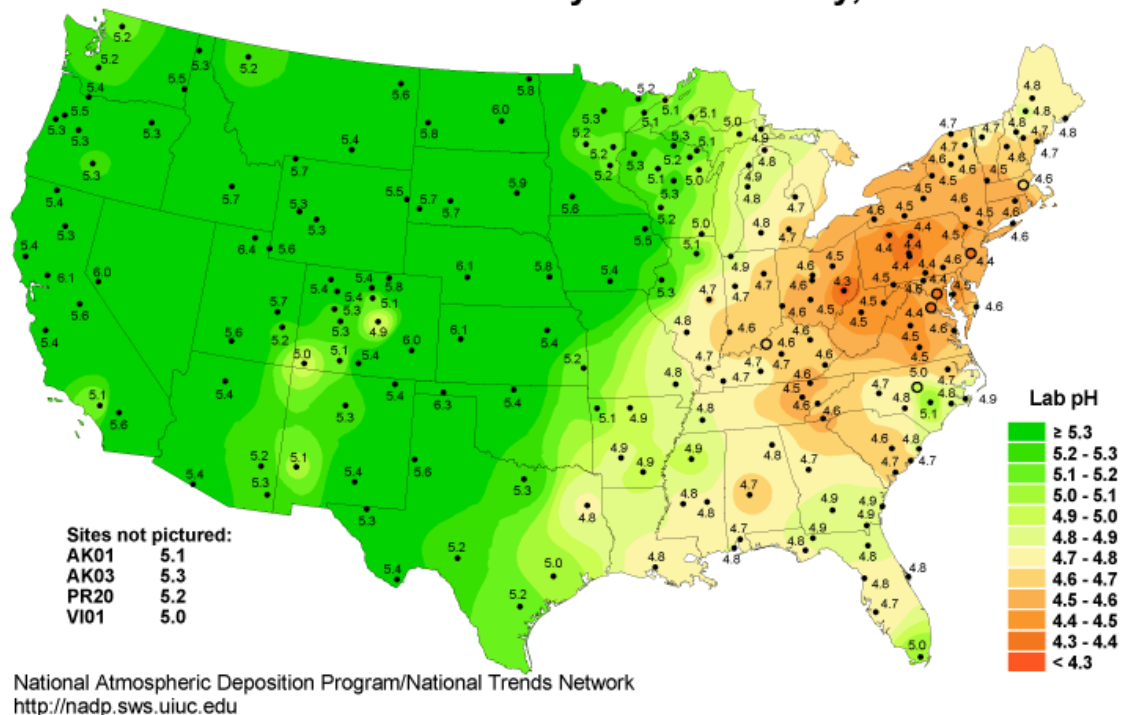
Figure 47: The pH isopleth map indicates that rainfall is more acidic in the East and Northeast regions of the United States, but monitoring has shown a decrease in acidity levels over time due to reductions in sulfur dioxide and nitrogen oxides. Map courtesy of the National Atmospheric Deposition Program.
