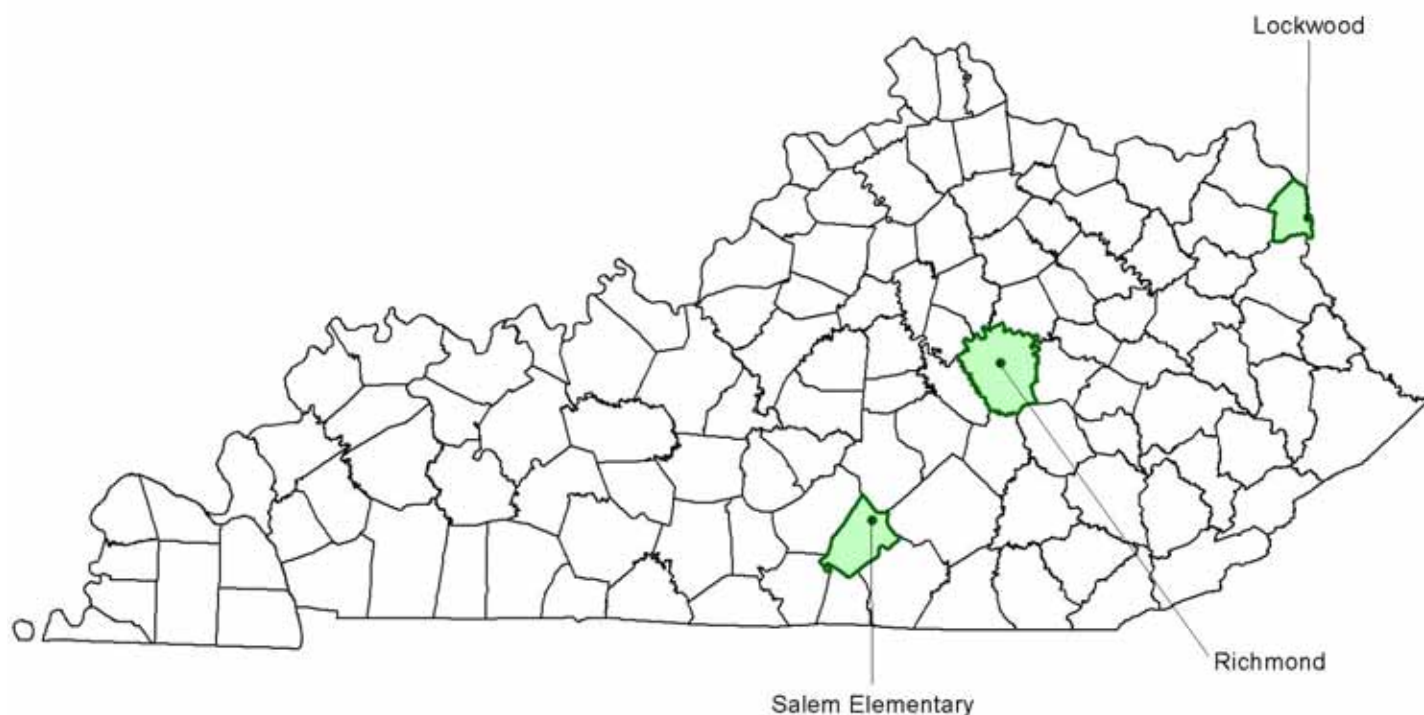
Figure 31: Proposed Lead monitoring locations in Kentucky.
