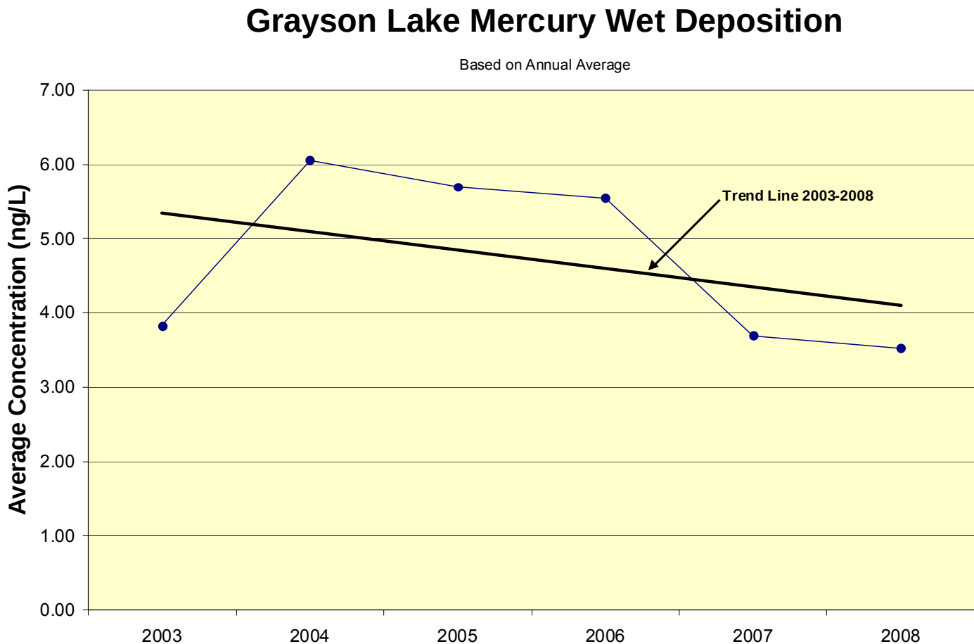
Figure 44: Grayson Lake averages for Hg monitoring indicate pollution reductions.
