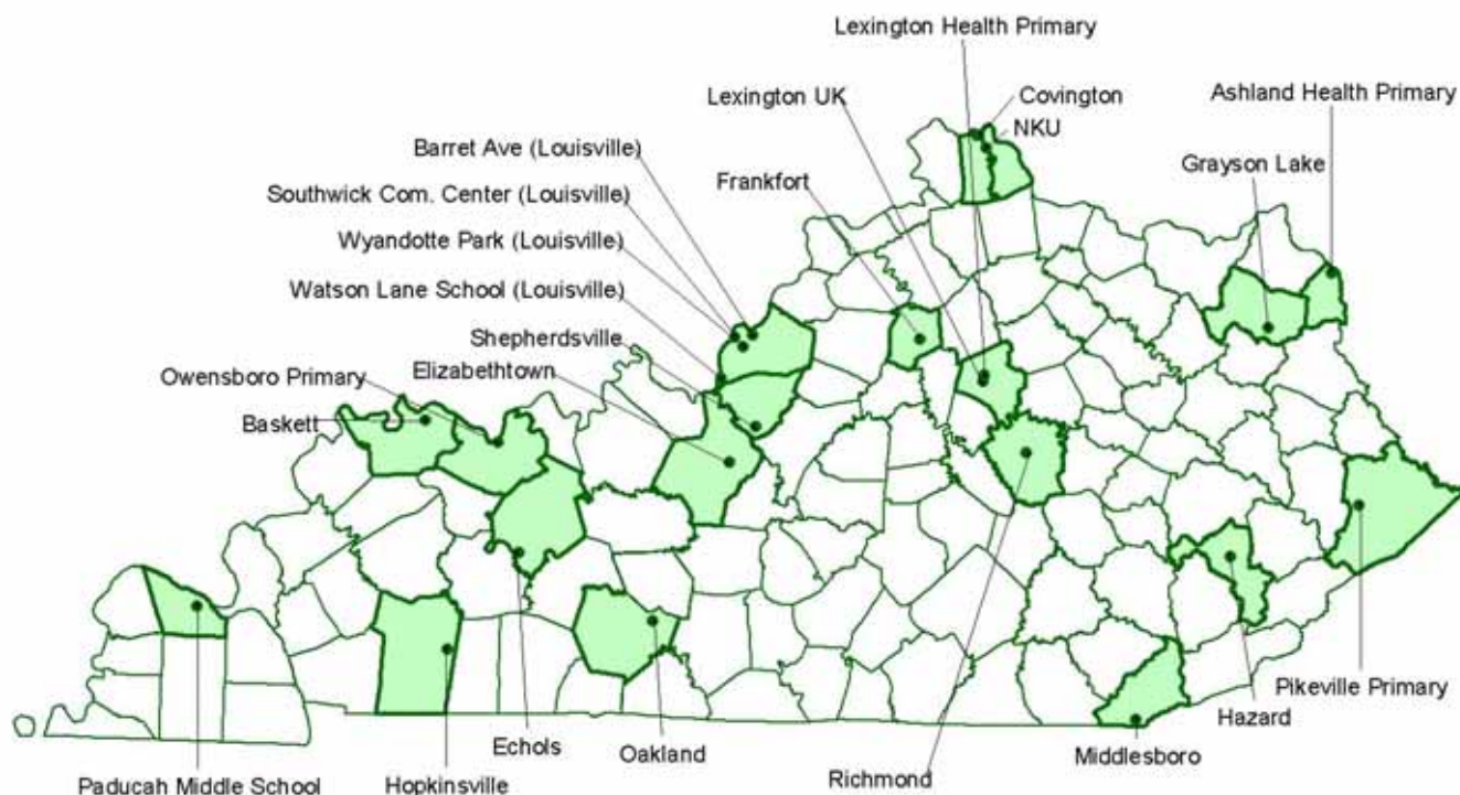
Figure 36: PM 2.5 monitoring locations in Kentucky.
