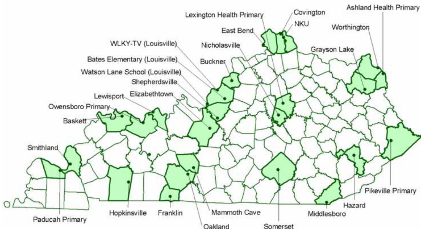
Figure 34: Ozone monitoring locations in Kentucky.
