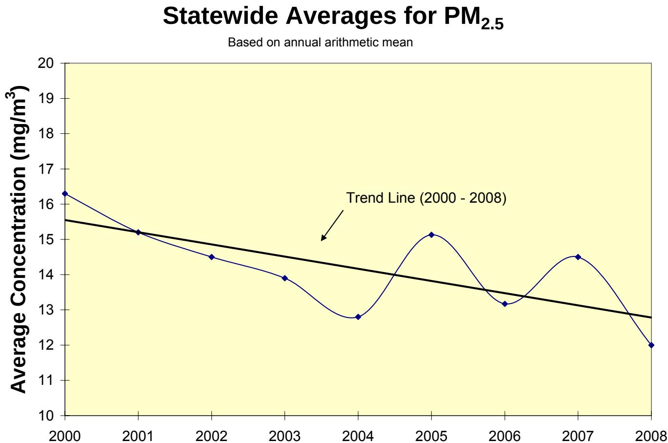
Figure 37: Statewide averages for PM_{2.5} monitoring indicate pollution reductions.
